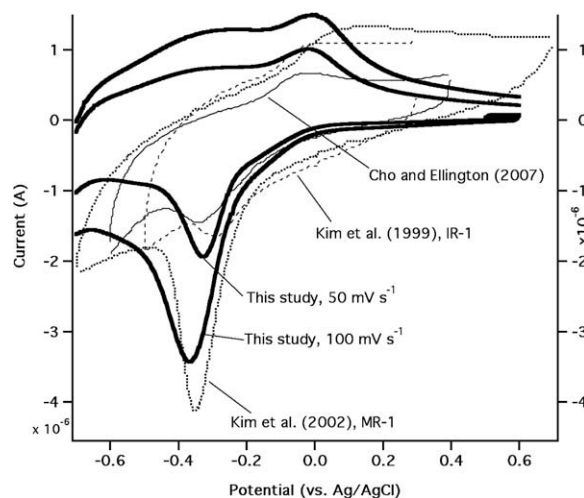
Fig. 6. Background-subtracted CV data for wild-type Shewanella oneidensis MR-1 under anaerobic conditions, at 50 mV s^{-1} (thick gray) and 100 mV s^{-1} (thick black) scan rates, compared with 100 mV s^{-1} data from other studies.
