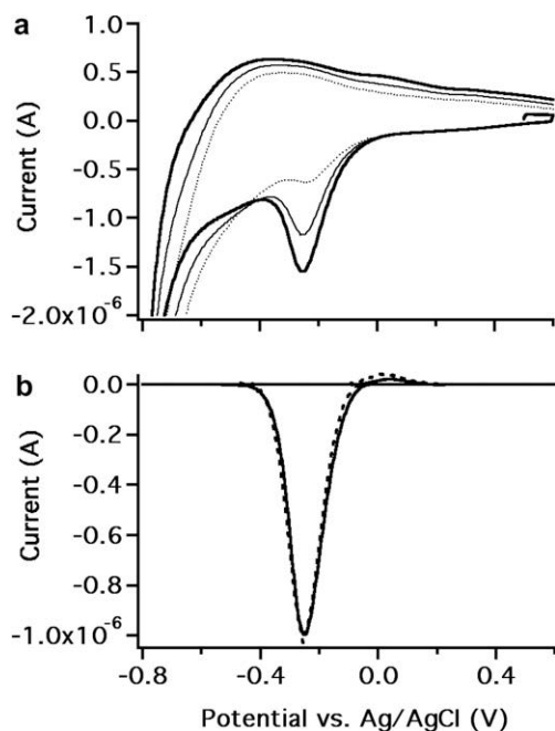
Fig. 9. (a) CV for \Delta mtrC\text{-}\Delta omcA under N_2 purging. Initial scan after 10 s hold (dotted), first 30 s hold (thin solid), and last 30 s hold (thick solid); all holds at +500 mV. (b) Background subtracted data from the last 30 s hold (solid) compared to CV of artifactual Fe (dashed). There is no evidence in the CV of \Delta mtrC\text{-}\Delta omcA for electron transfer between hematite and any redox-active species other than Fe dissolved from the electrode.
