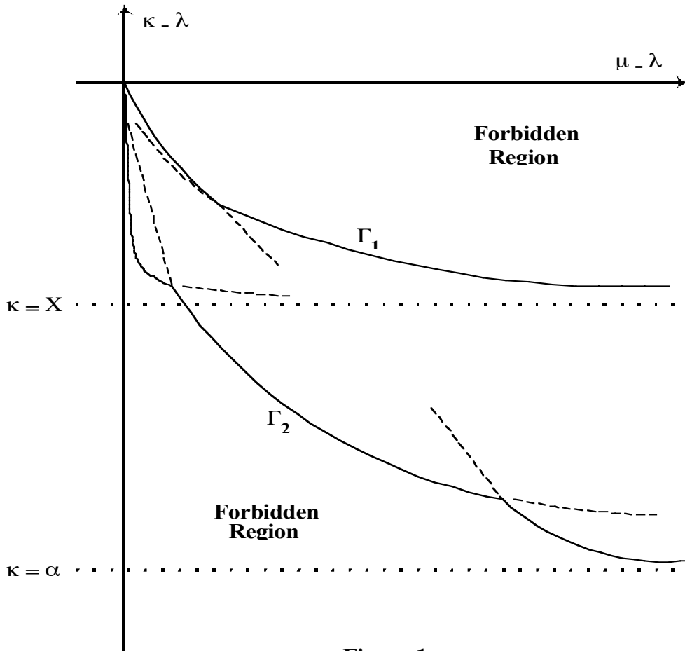
Figure 1 Locus of the Inclusion Intervals (\kappa, \mu) \kappa = \mathbf{m}(\mathbf{x}) \quad \mu = \mathbf{M}(\mathbf{x}) \Gamma_1: \kappa = \Phi^{-1}(\mu) \quad \Gamma_2: \kappa = \psi(\mu)
