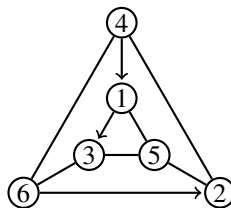
FIGURE 4.1. The mixed graph for Example 4.1.
