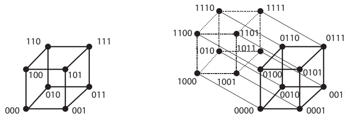
FIGURE 1. The hypercubes Q_3 and Q_4 .
