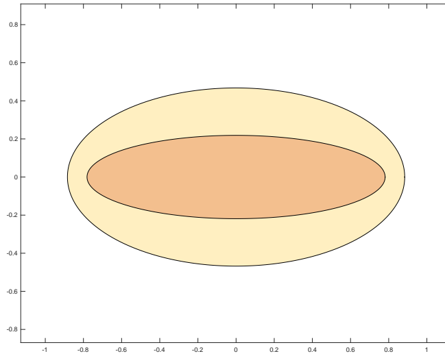
FIGURE 8. \mu = -\lambda = 3/4 . The numerical range and maximal numerical range are both elliptical discs.
