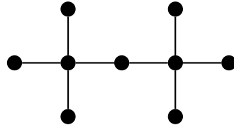
FIG. 2.2. A tree with degree sequence \pi = (4^2, 2^1, 1^6) where no BFD-ordering exists.
