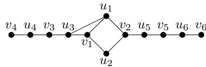
Fig. 6.2: The graph S_{4,4} with a single edge added. The parameter q for this graph is at least 10.
