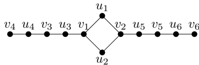
Fig. 6.1: The graph S_{4,4} and q(S_{4,4}) = 6 .
