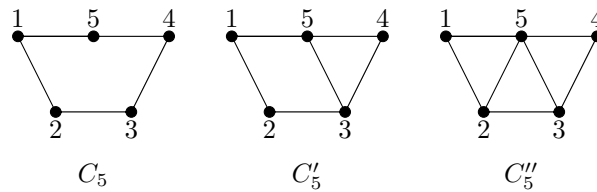
Fig. 7.1: Base exceptional graphs.
