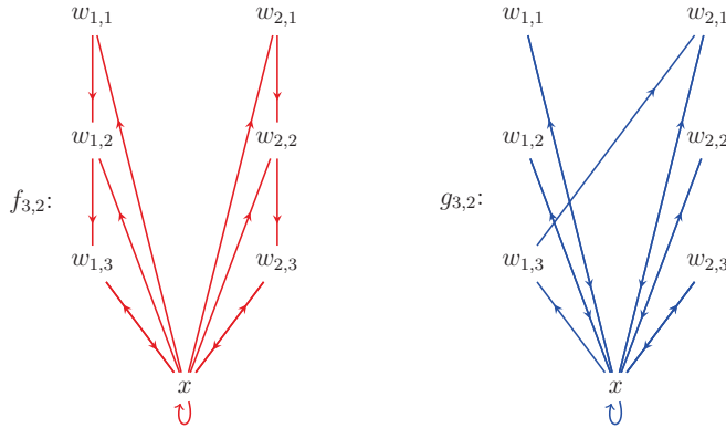
FIG. 3.1. The two digraphs f_{3,2} and g_{3,2} as described in Example 3.3.
