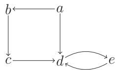
FIG. 1.3. A digraph f for which \mathcal{PS}_f contains a path of length L_f > D_f ending at a singleton set.
