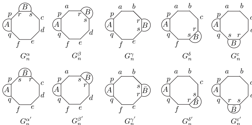
FIGURE 4. Graphs G_n^\alpha, G_n^\beta, G_n^\gamma, G_n^\delta, G_n^\varepsilon and G_n^{\alpha'}, G_n^{\beta'}, G_n^{\gamma'}, G_n^{\delta'}, G_n^{\varepsilon'} .
