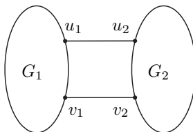
FIGURE 3. Graph G_1 \diamond G_2 .
