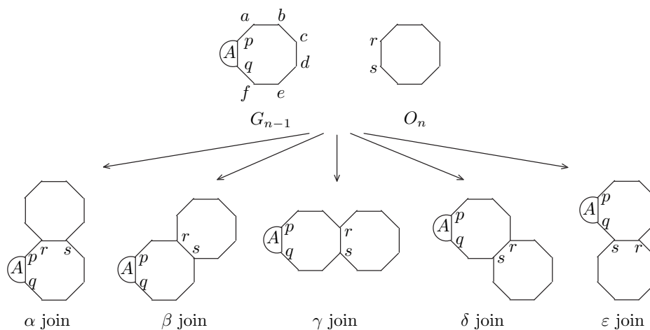
FIGURE 1. Five cases of attaching an octagon O_n to an octagonal chain G_{n-1} .
