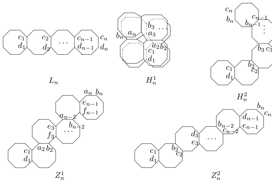
FIGURE 2. Graphs L_n , H_n^1 , H_n^2 , Z_n^1 and Z_n^2 .
