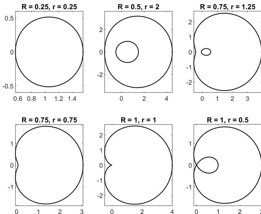
FIGURE 1. Cartesian ovals for products of complex circles with center 1 and radii R and r .
