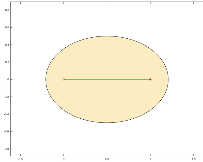
FIGURE 2. A = \begin{bmatrix} 1 & i \\ 0 & 0 \end{bmatrix} ; z_0 coincides with one of the eigenvalues since the other is zero.
